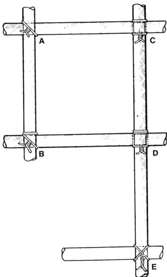
Figure 19: Common rebar ties. (A) Single tie, (B) Wrap and single tie, (C) Saddle tie, (D) Wrap and saddle tie, (E) Figure-eight tie. Courtesy of the Reinforcing Steel Institute of Ontario.
