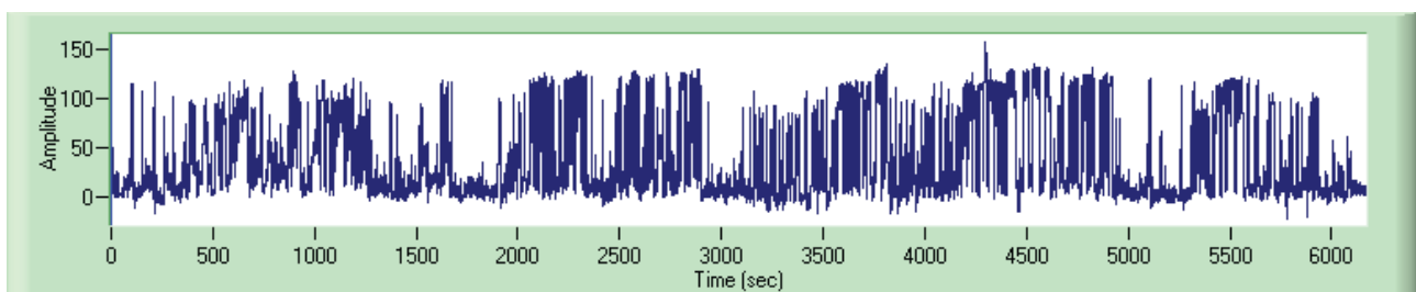
Figure 8: Field collected trunk flexion/extension angles (flexion is positive scale) while performing rebar work using pliers. The median trunk posture across the data collection period was 42.6 flexion. All data were collected using a mobile 3DM-G gyroscope.
