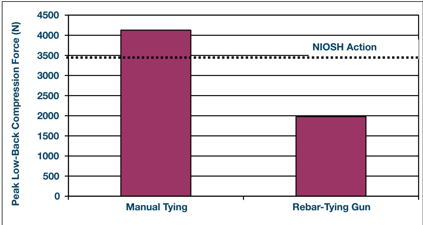
Figure 7: Tying with rebar tying gun resulted in significant ( p=.018 ) decrease in peak loading on the lower-back (L4/L5 disc). Manual tying exposed workers to peak compression force loading that is greater than NIOSH Action Limit (3400 N).
