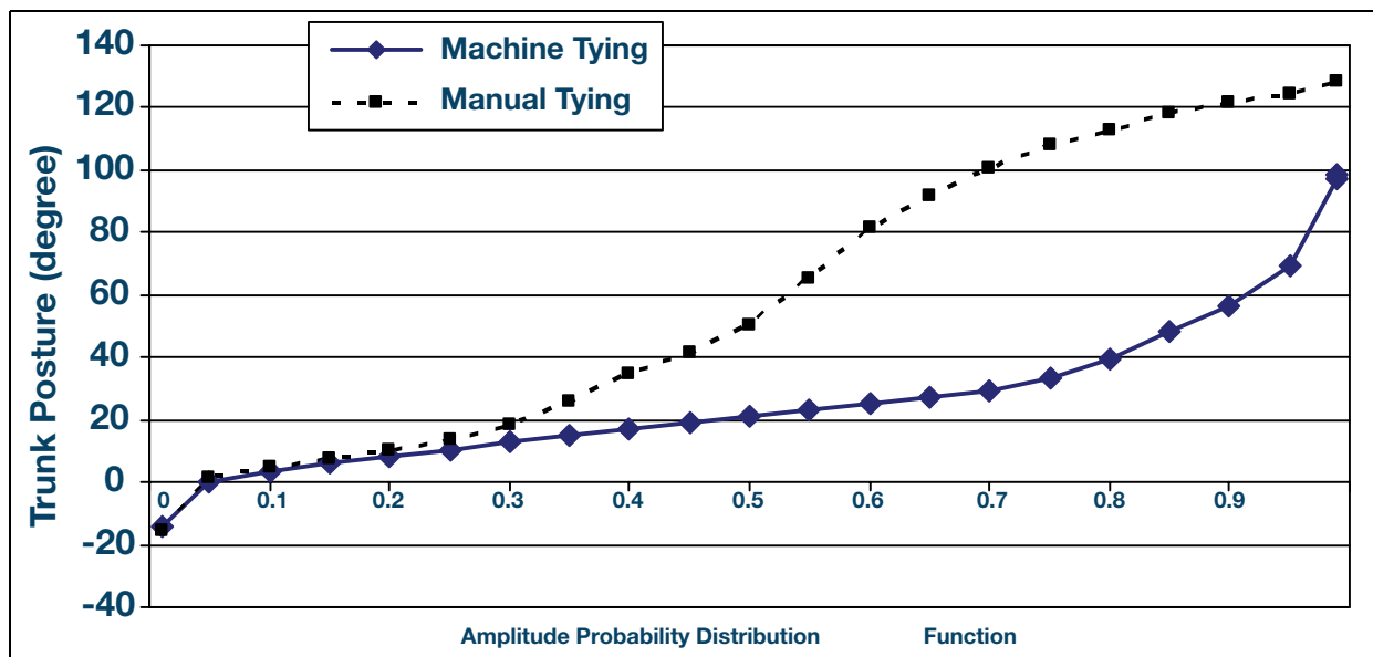
Figure 13: Average APDF of the trunk posture. Average values were obtained from individual APDF curves from Figure 14 and 15.
