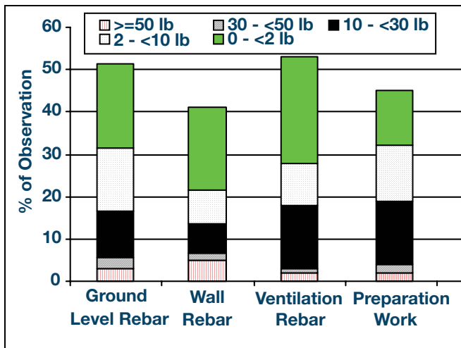
Figure 3: Frequency of loads handled by task among rodworkers. Reproduced from Paquet et al (1999).
