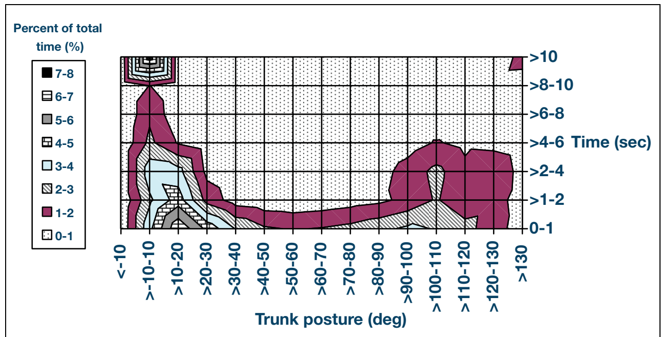
Figure 11: A contour graph detailing trunk posture while tying with pliers.
