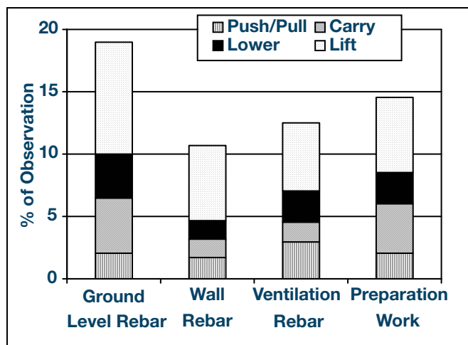
Figure 2: Frequency of manual material handling activities by task among rodworkers. Reproduced from Paquet et al (1999).
